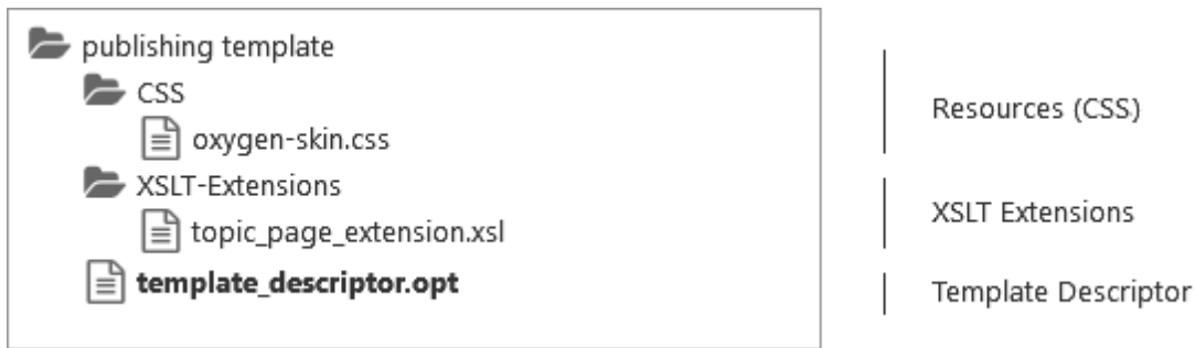
Figure 316. Oxygen Publishing Template Package (PDF)
