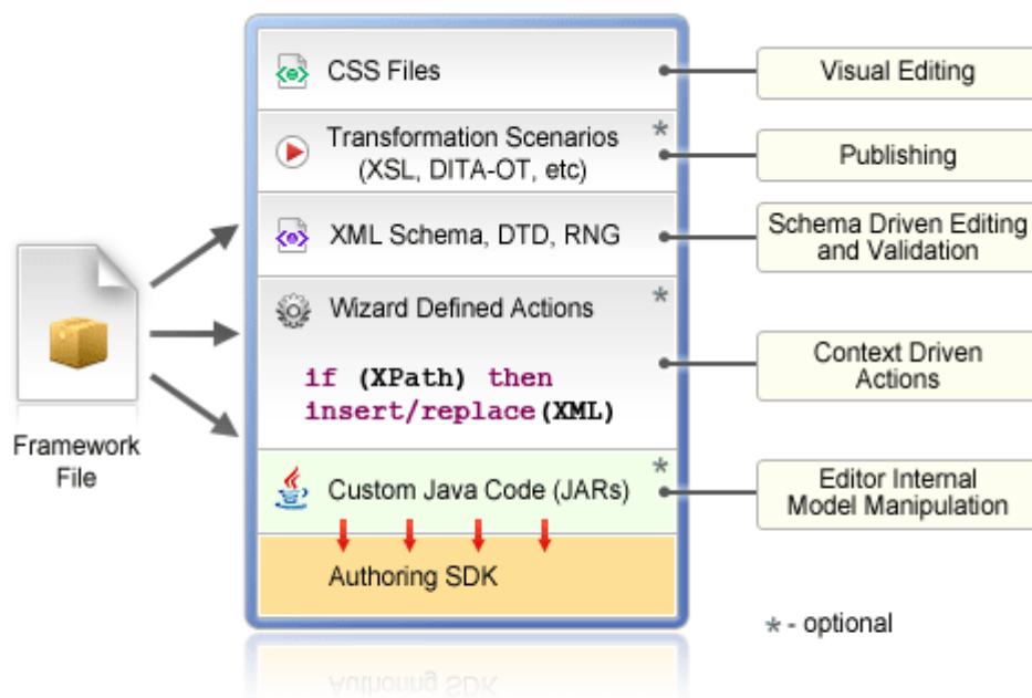
Figure 390. Components of a Custom Framework
