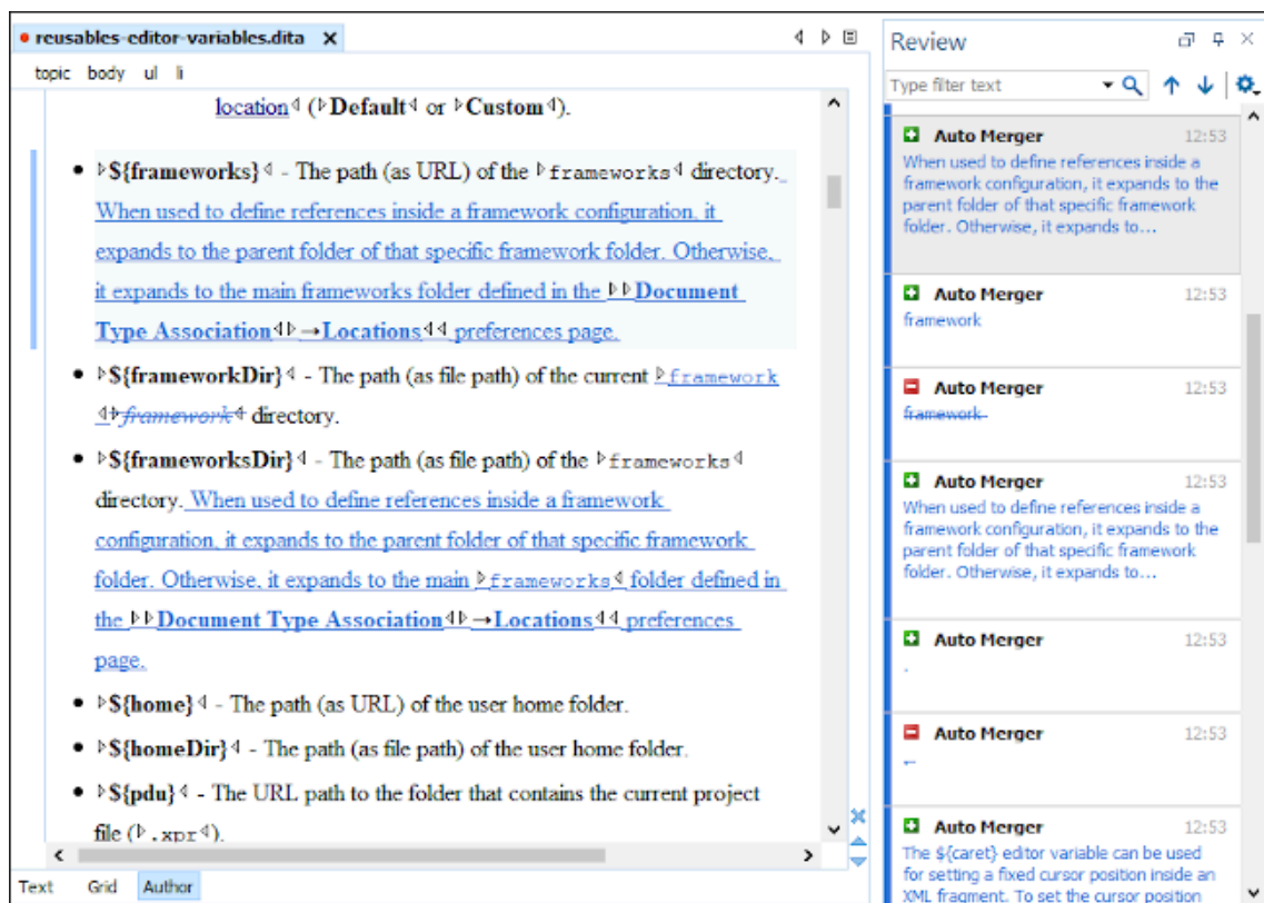
Figure 568. Example of a Merged File with Change Tracking Markers Opened in Author Mode
