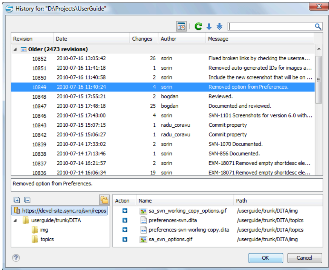
Figure 439. History Dialog Box
