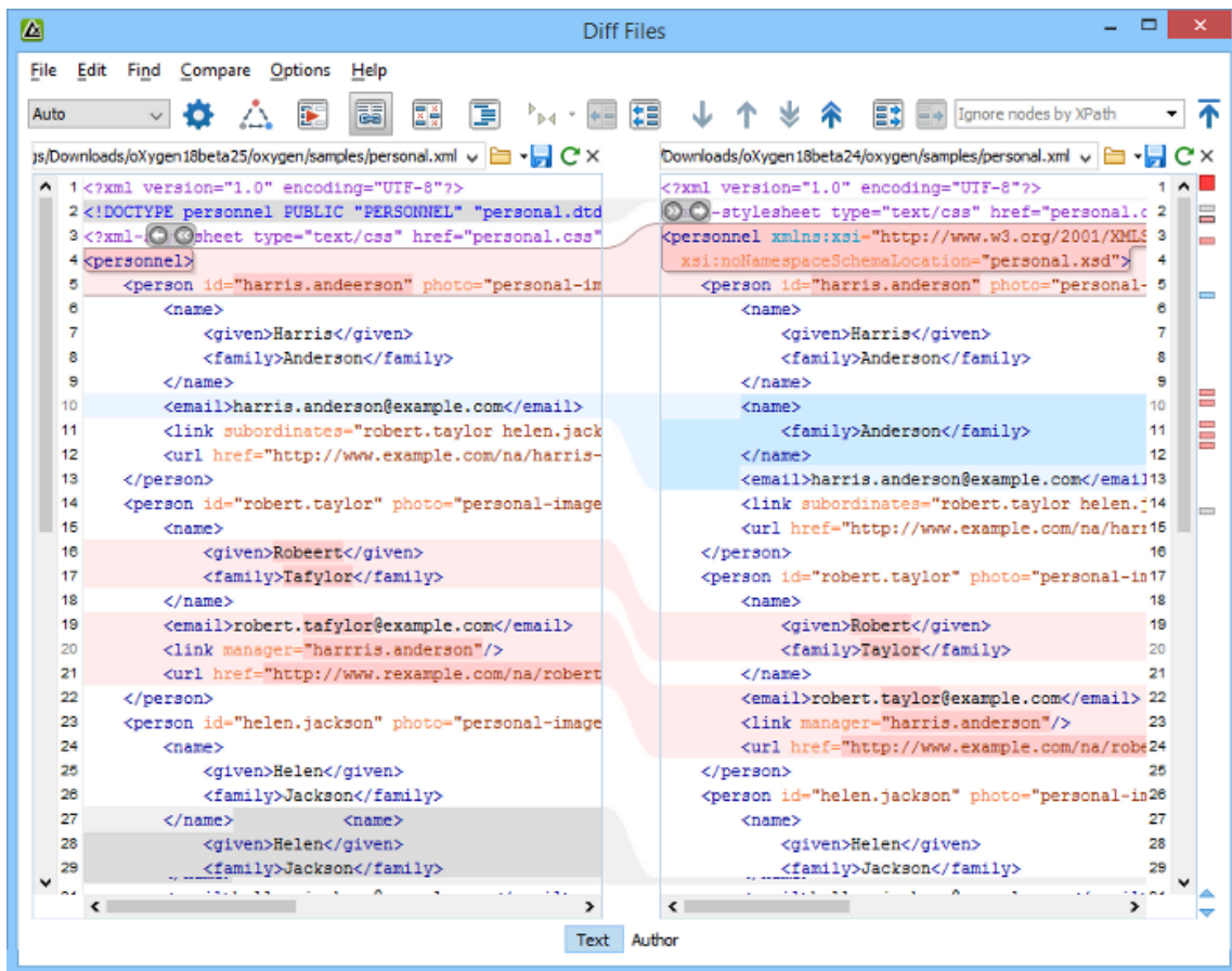
Figure 409. Compare Files Tool
