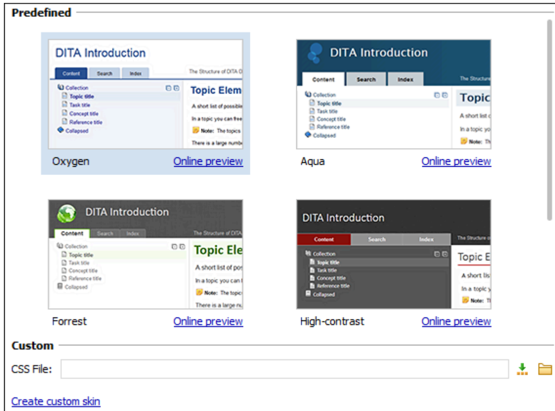
Figure 276. Skins Tab
