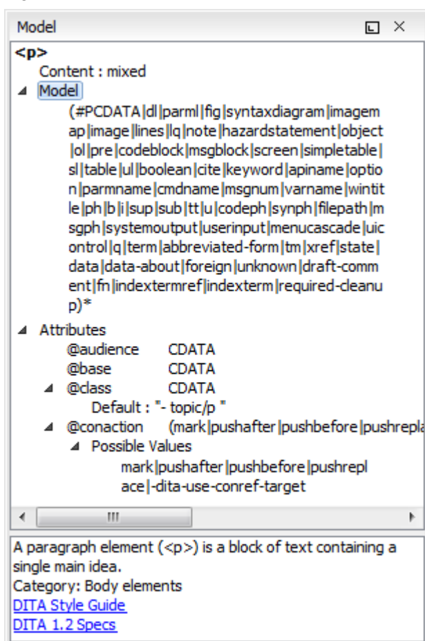
Figure 119. Model View
