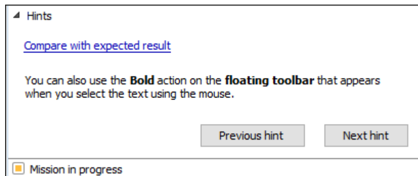
Figure 399. Hints Pane
