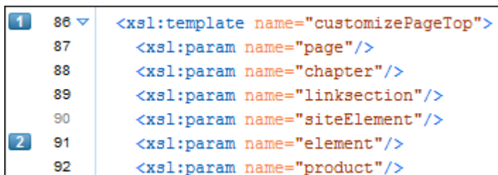
Figure 112. Editor Bookmarks
