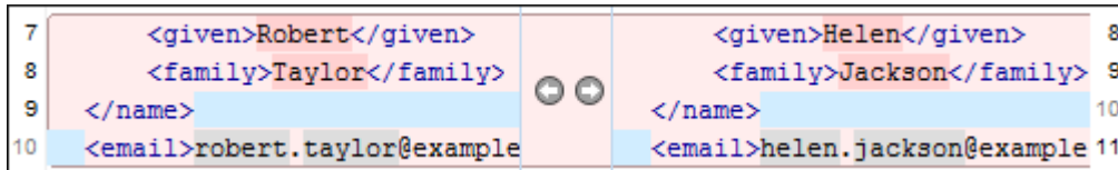
Figure 412. Three-Way Differences
