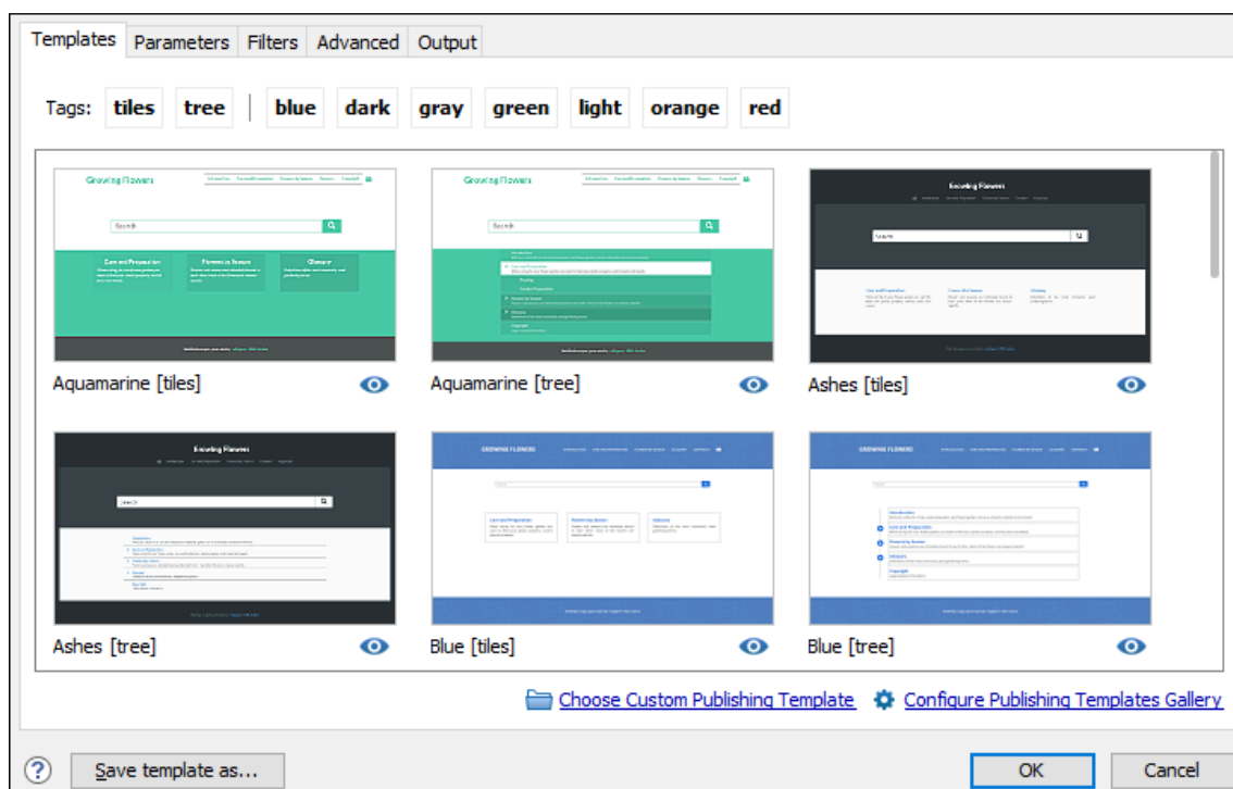
Figure 277. Templates Tab
