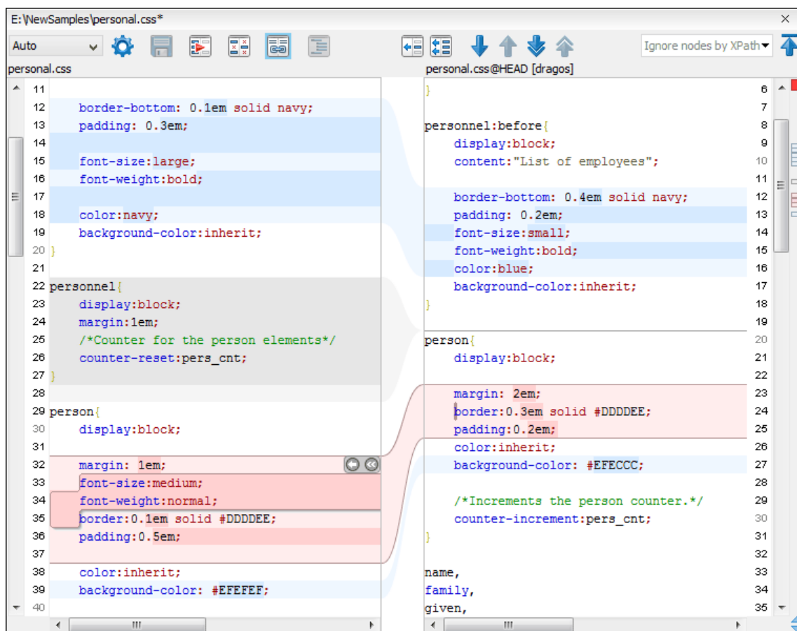
Figure 476. Compare View
