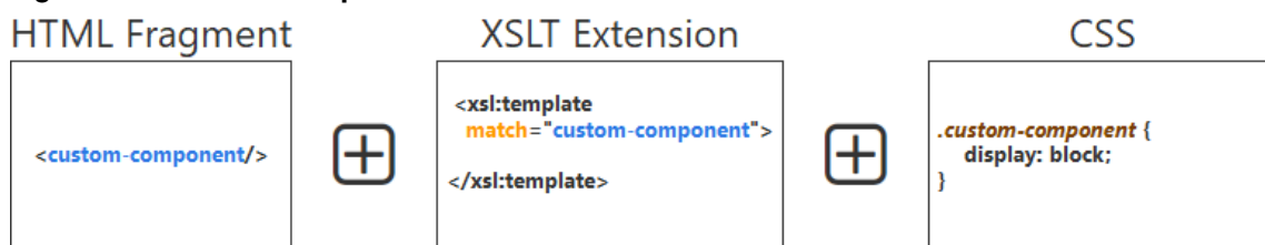
Figure 309. Custom Component
