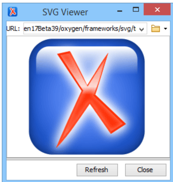
Figure 255. SVG Viewer
