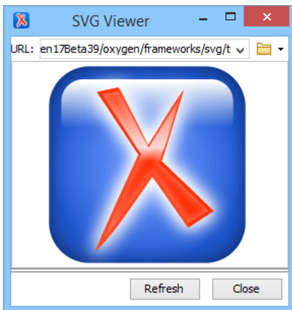
Figure 408. SVG Viewer
