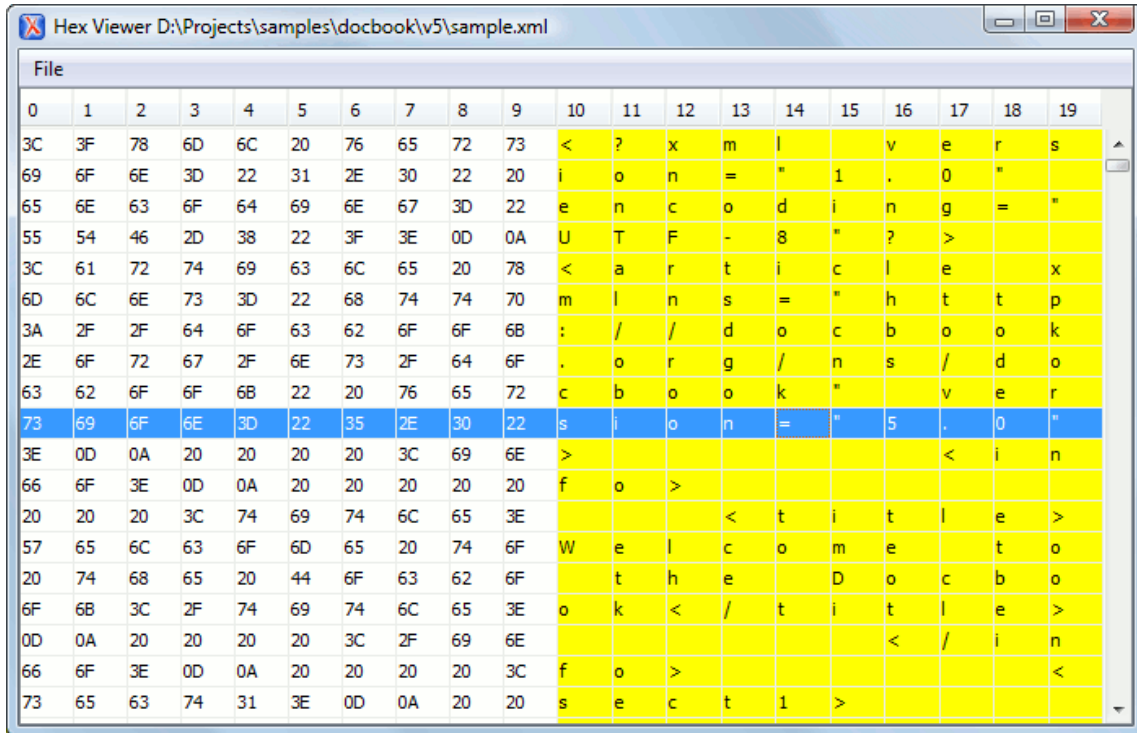
Figure 407. Hex Viewer
