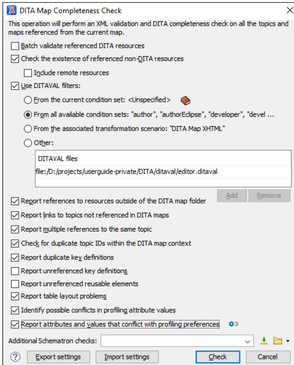
Figure 503. DITA Map Completeness Check Dialog Box
