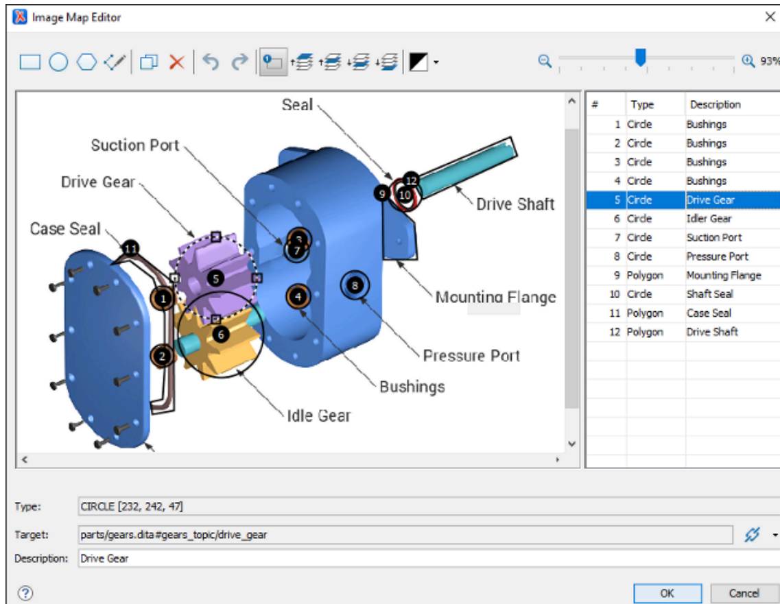
Figure 511. Image Map Editor in DITA
