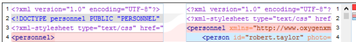
Figure 410. Two-Way Differences
