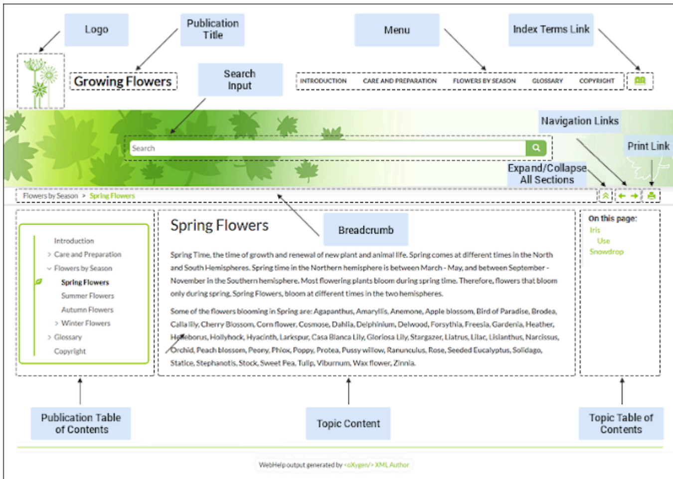
Figure 291. Topic Page
