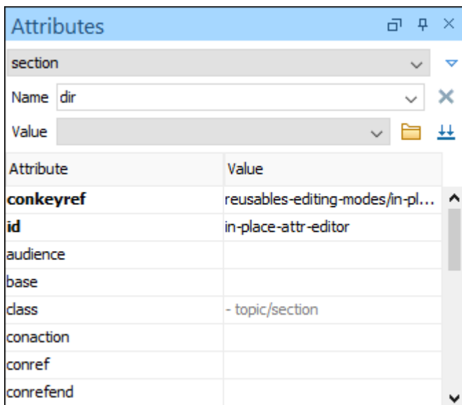
Figure 118. Attributes View
