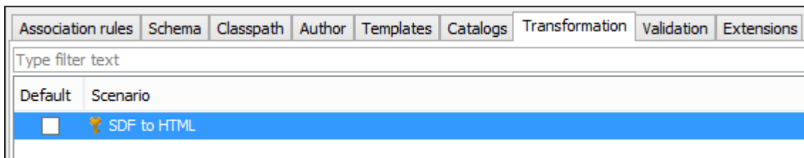
Figure 367. Transformation Tab
