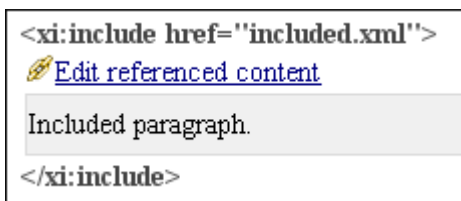
Figure 140. XInclude reference
