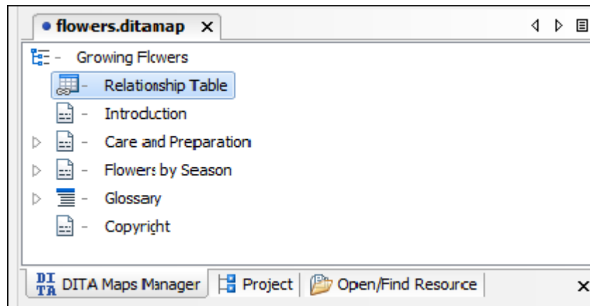
Figure 540. Relationship Table
