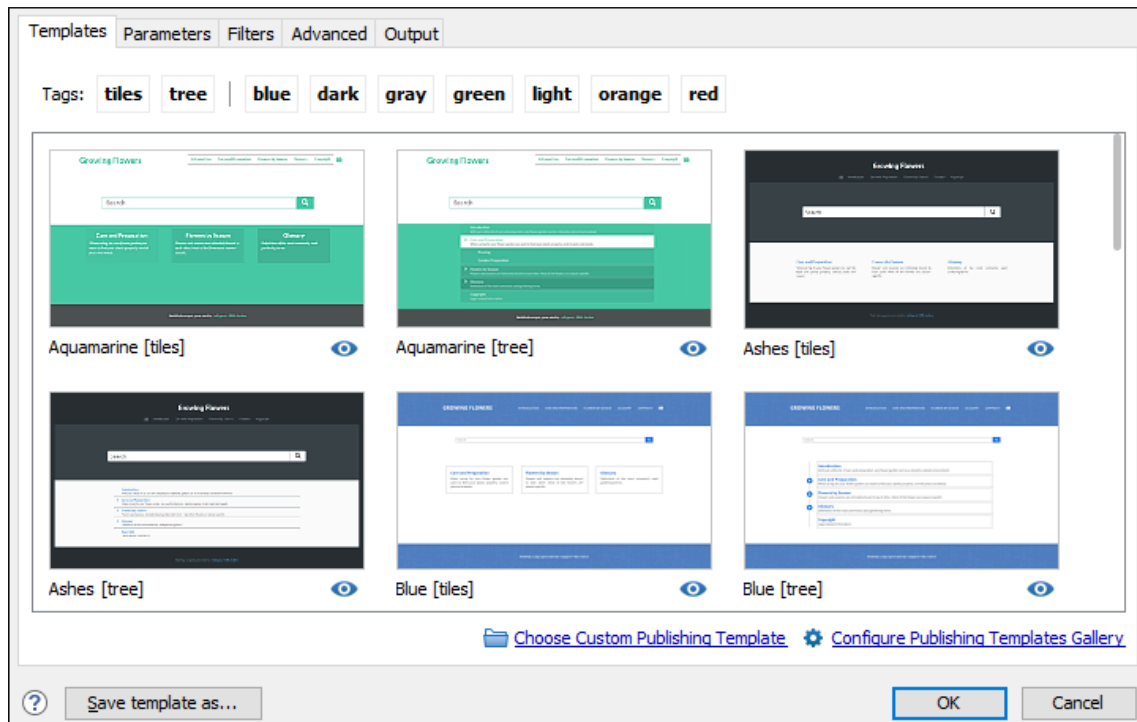
Figure 543. Templates Tab
