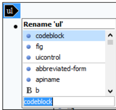
Figure 152. Example (Rename)
