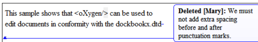
Figure 174. Deletion Callouts
