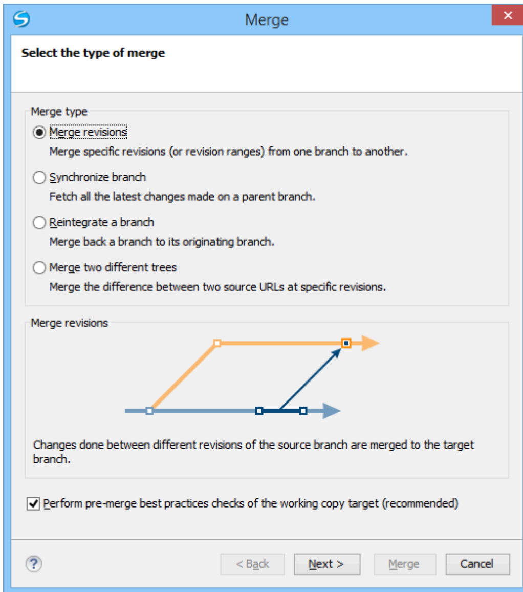
Figure 447. Merge Wizard
