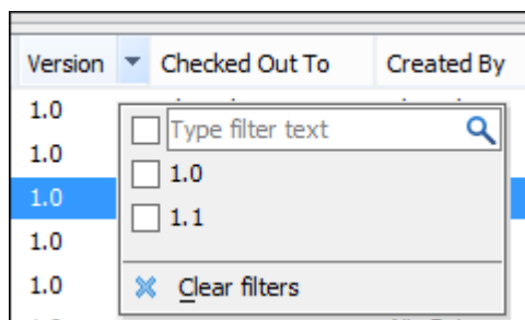
Figure 67. Column Filter
