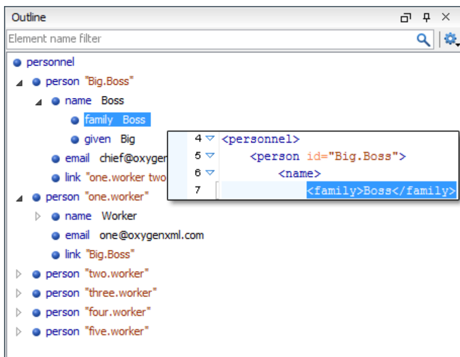
Figure 117. Outline View
