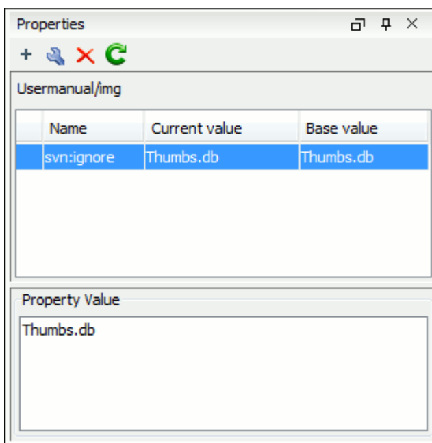
Figure 478. Properties View
