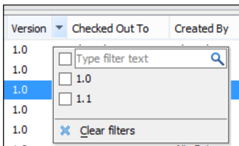
Figure 348. Column Filter
