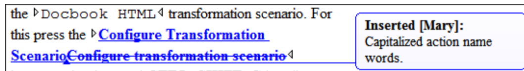
Figure 175. Insertion Callouts
