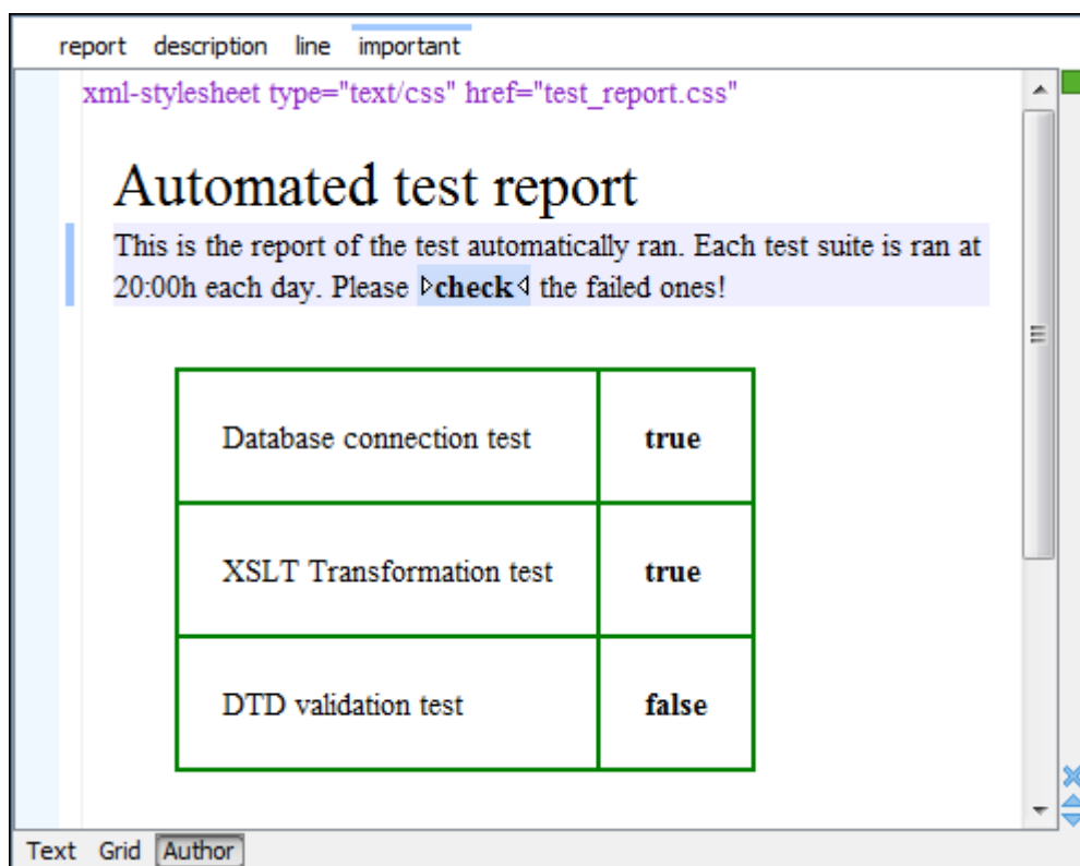
Figure 382. Report Rendered in Author Mode
