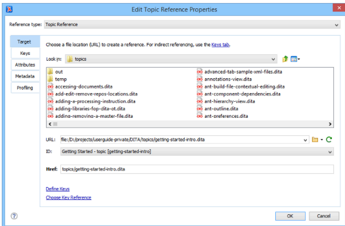
Figure 771. Edit Properties Dialog Box - Target Tab
