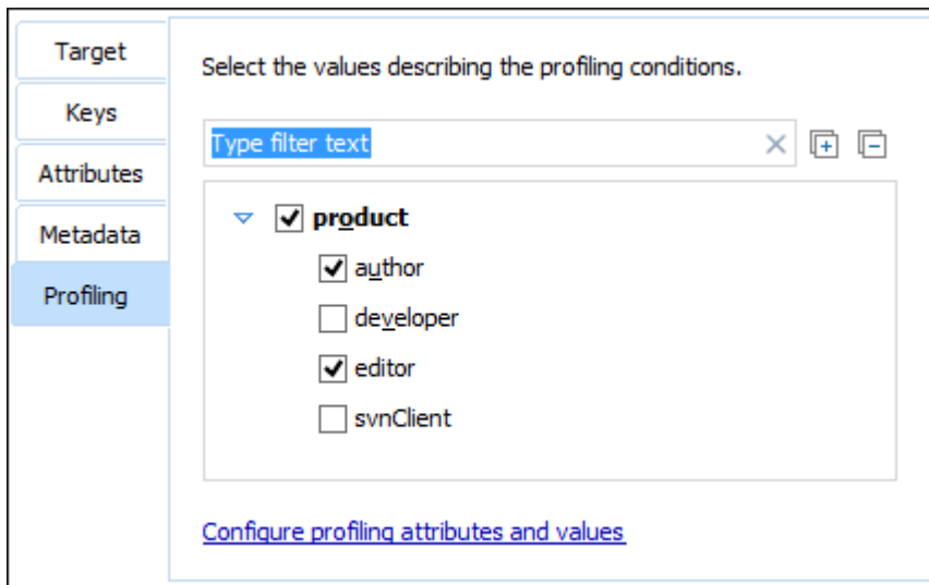
Figure 768. Insert Reference Dialog Box - Profiling Tab
