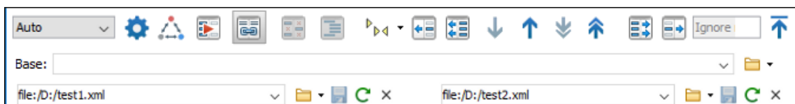
Figure 98. Compare Toolbar
