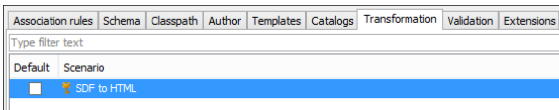
Figure 598. Transformation Tab
