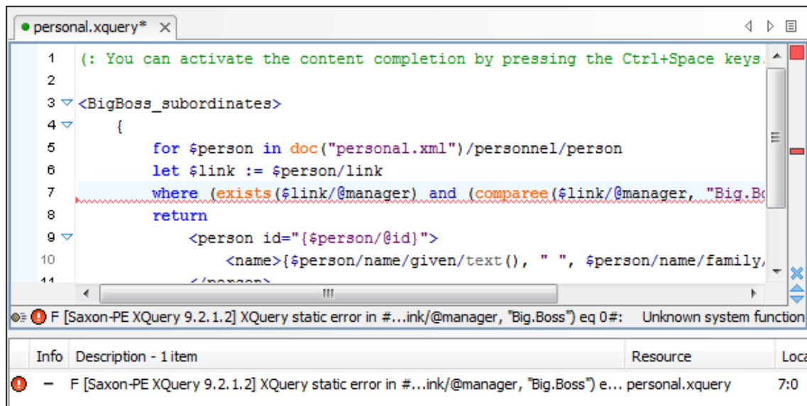
Figure 354. XQuery Validation
