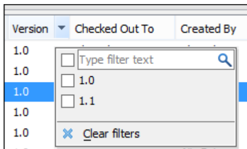
Figure 68. Column Filter
