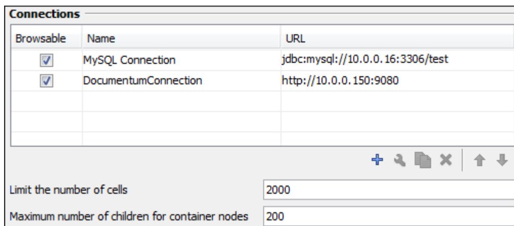
Figure 36. Connections Preferences Panel
