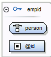
Figure 323. The xs:key Component
