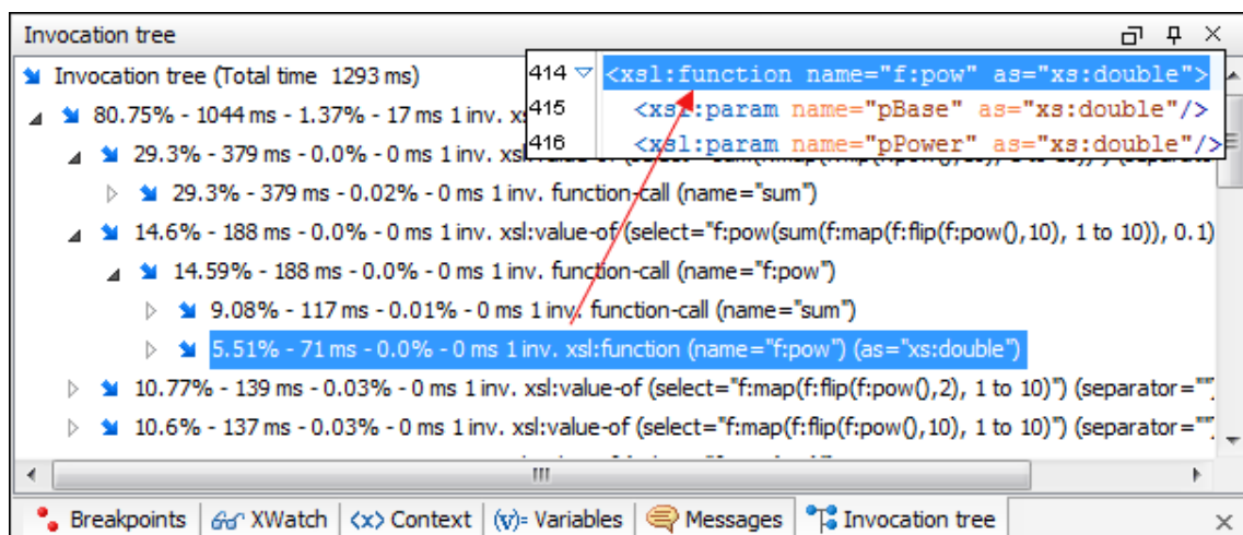
Figure 582. Source Backmapping
