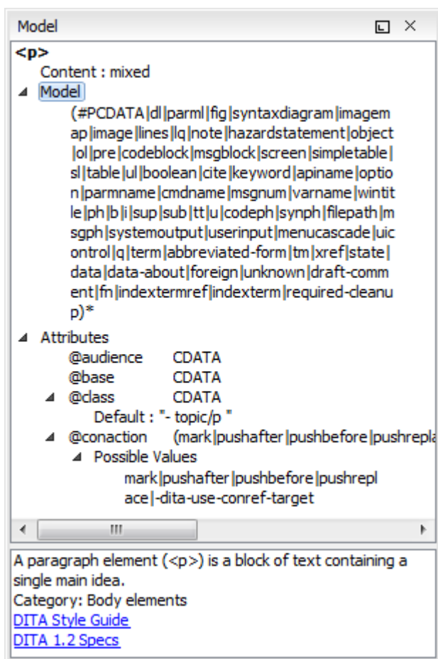
Figure 161. Model View
