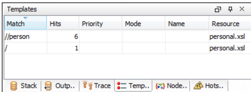
Figure 576. Templates view
