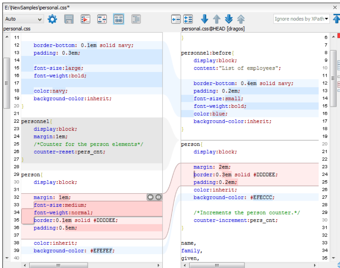
Figure 751. Compare View
