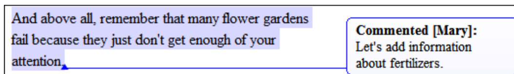
Figure 173. Comment Callouts
