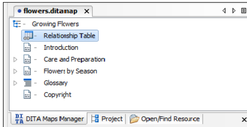
Figure 815. Relationship Table
