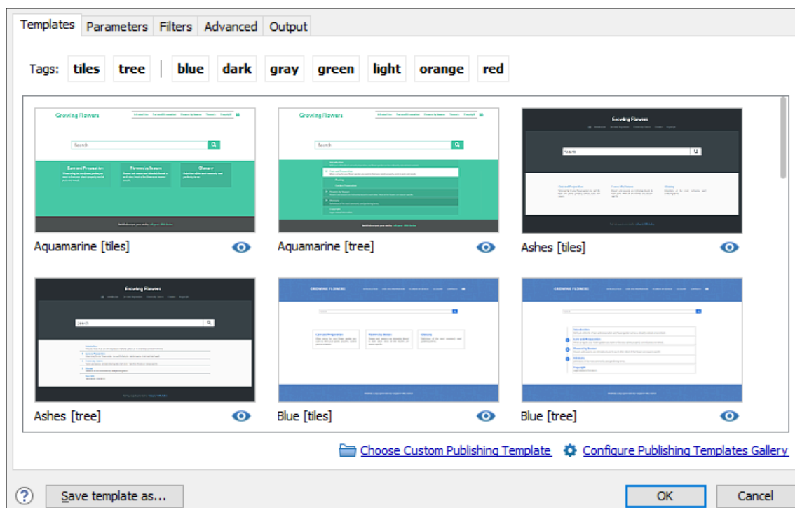
Figure 486. Templates Tab
