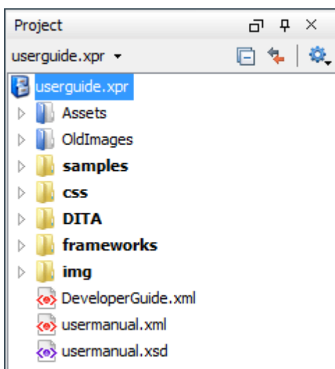
Figure 71. Project View
