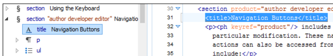
Figure 110. Outline View Navigation in Text Mode
