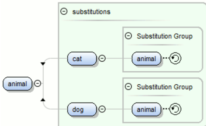
Figure 331. Substitutions Construct
