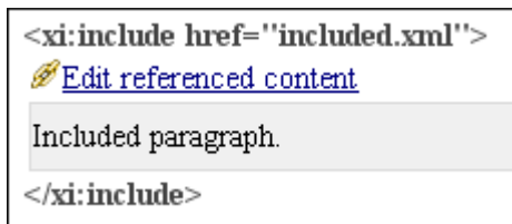
Figure 141. XInclude reference
