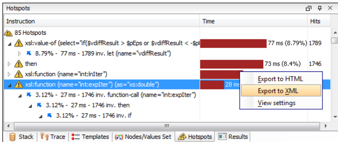
Figure 584. Hotspots View
