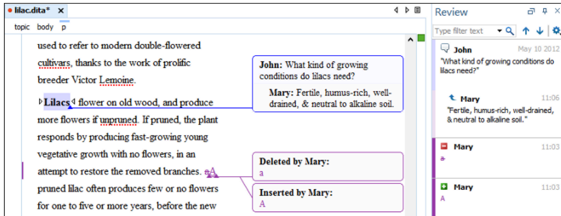
Figure 177. Review View
